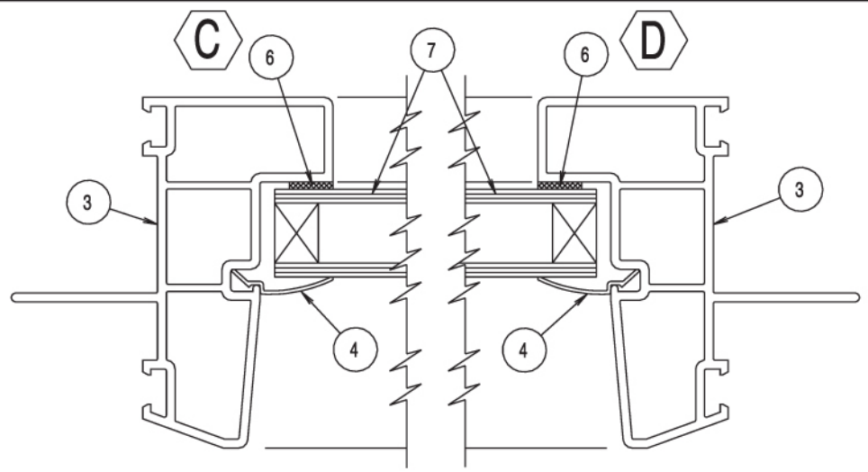
HORIZONTAL SECTION
