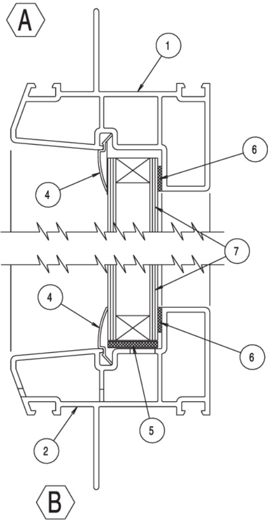
VERTICAL SECTION
